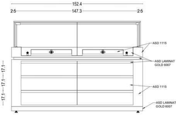
1 FRONT VIEW
