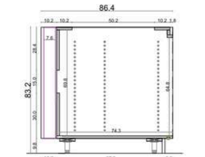
A-A SECTION OF CABINET BODY
