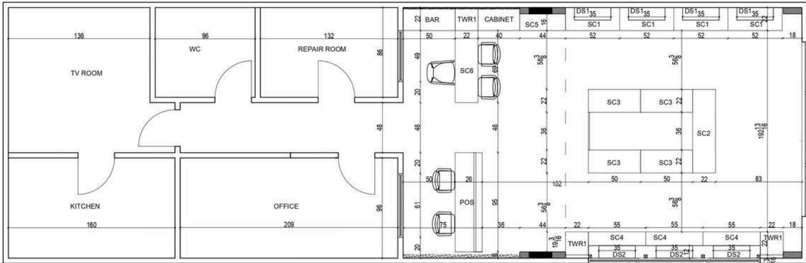
1 LAYOUT PLAN
